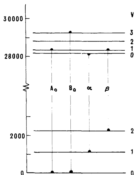
Figure 7. The \nu_4' and \nu_4'' manifolds of levels in the \tilde{X}^1A_1 and \tilde{A}^1A_2 electronic states of formaldehyde. The notation of Brand 10 has been used to denote the transitions.
