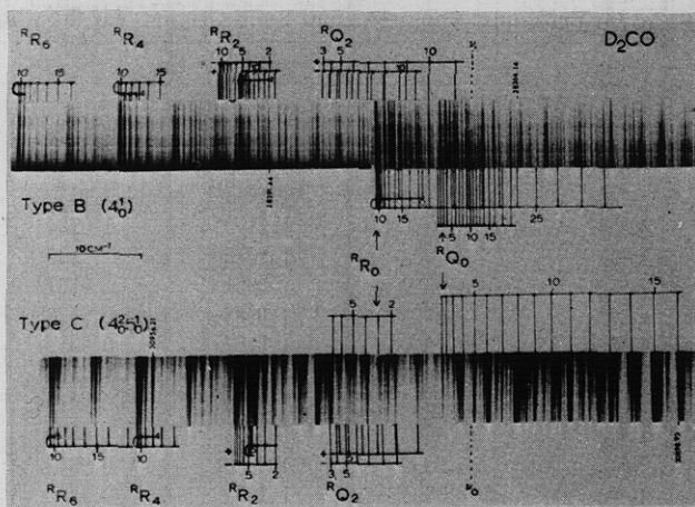
Figure 10. Central portions of two perpendicular bands of \text{D}_2\text{CO} . The type-b 4_0^1 band centered at 28,369.44 \text{ cm}^{-1} and the type-c 4_0^25_0^1 band at 30,921.54 \text{ cm}^{-1} (Job, Sethuraman, and Innes, ref 42).
