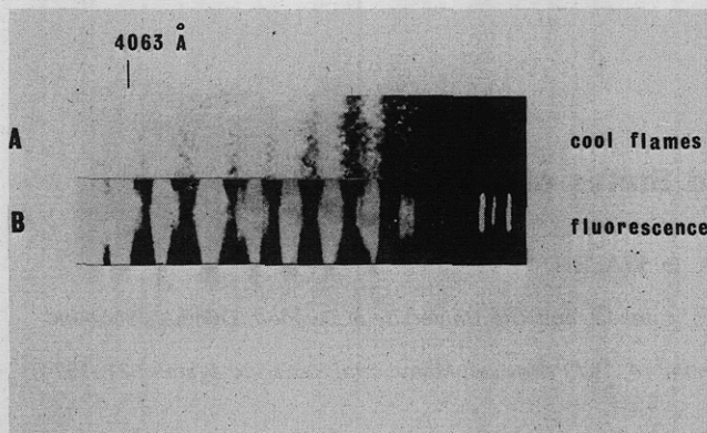
Figure 1. (A) The spectrum of the cool flame of diethyl ether as photographed by Emeléus. 3 (B) Part of the fluorescence spectrum of formaldehyde as obtained by Gradstein. 6
