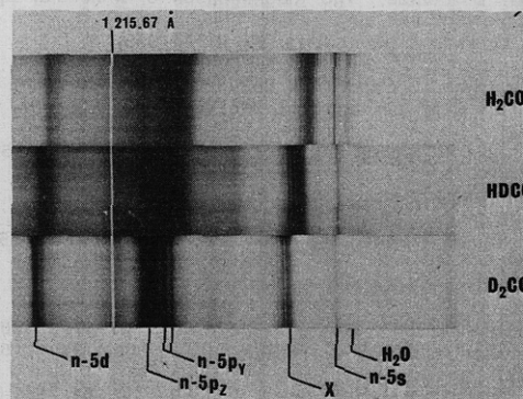
Figure 15. Absorption spectra of \text{H}_2\text{CO} , \text{HDCO} , and \text{D}_2\text{CO} in the 1240-Å region, recorded with 3-m McPherson spectrograph (Moule and Bell, ref 92).
