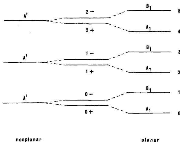
Figure 6. Energy levels of the nonrigid formaldehyde molecule. The symmetry of the electronic wave function is that of the \tilde{X}^1A_1 ground state.
